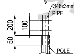
DOUBLE ARM DETAILS (90°)
