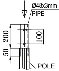
DOUBLE ARM DETAILS (60°)
